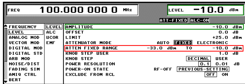
Fig. 2-1 The attenuator fixed range of the ATTENUATOR MODE FIXED is displayed in the ATTEN FIXED RANGE submenu section. Submenu section AMPLITUDE and LEVEL display, indicate the reference level for the ATTENUATOR MODE FIXED.
